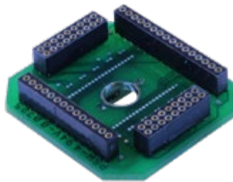
ADPT-EIB-54-Kopf-HS-36 Input: Mill-Max 14/16/18 socket Output: Omnetics 44 pin X 2
