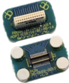
ADPT-EIB-16-QC-HS-16 Input: QuickClip 16 Output: Omnetics 26 pin
